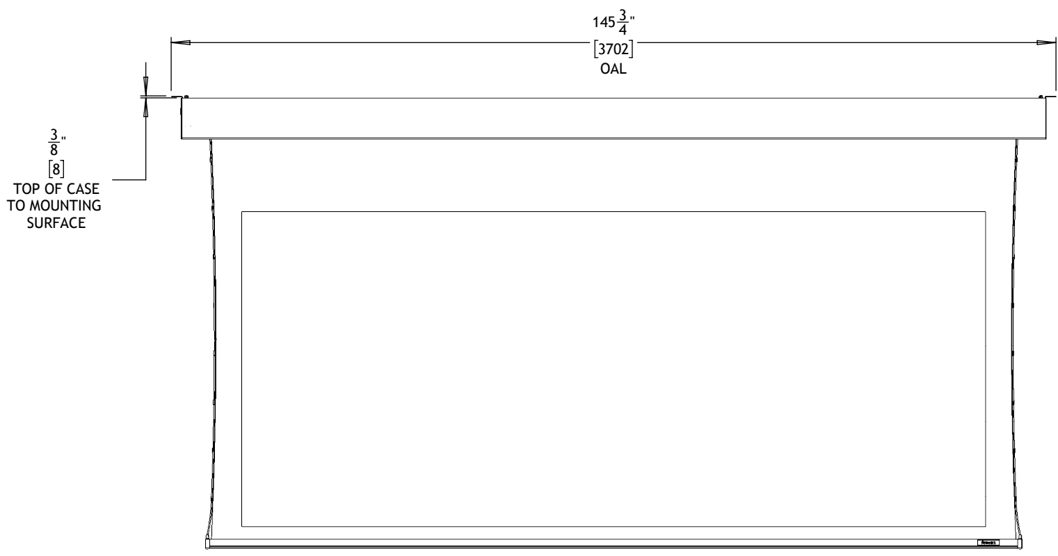
FRONT VIEW - CEILING MOUNT
