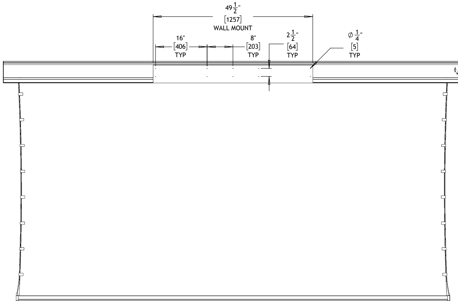
BACK VIEW - WALL MOUNT
